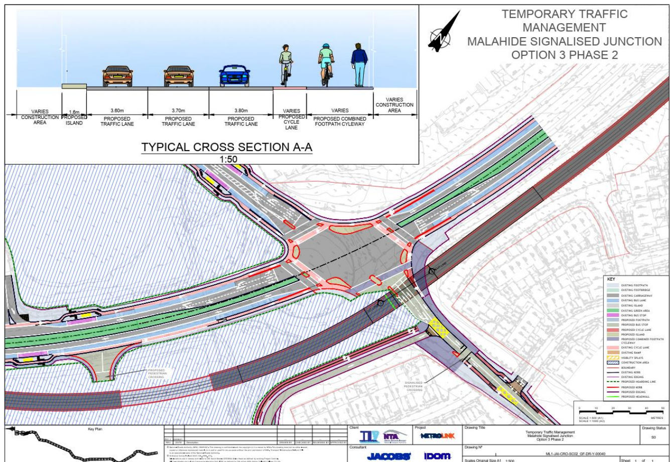
Figure 2: R132 / Malahide Road Signalised Junction Phase 2 Temporary Traffic Management
